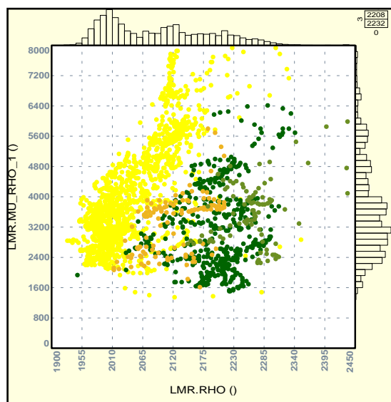
Figure 1: Log density vs \mu \cdot \rho with points coloured by core facies.
